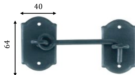
Art. 2133/ Chiavistello/Cabin hook A 145mm- Asta/Hook 100mm B 195mm- Asta/Hook 150mm
