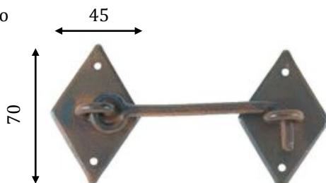
Art. 2132/ Chiavistello/Cabin hook A 145mm- Asta/Hook 100mm B 195mm- Asta/Hook 150mm
